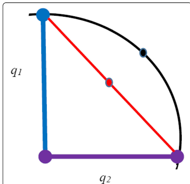
Fig. 4 Spherical interpolation between the quaternions, q_1 and q_2 . If simple linear interpolation was used then the interpolated point would be based on a line passing through the hypersphere (the red colored chord). Using spherical interpolation, the predicted point is on the surface of the hypersphere
