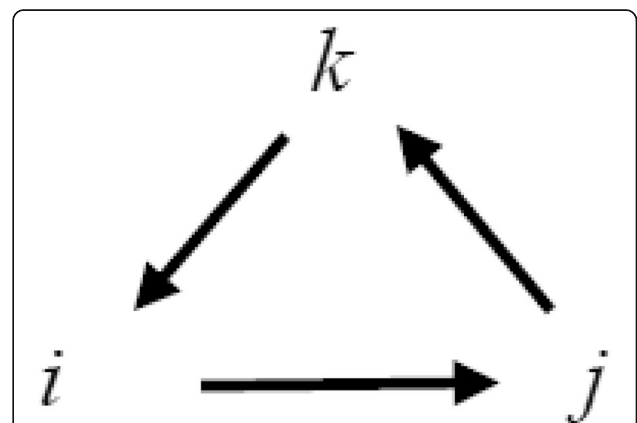
Fig. 1 Products of imaginary numbers comprising a quaternion. Given any starting point, moving in a counter-clockwise direction (with the arrows) gives the results of the products of the imaginary numbers (e.g., k,i=j ). If the motion is clockwise then the product is negative (e.g., j,i=-kj )
